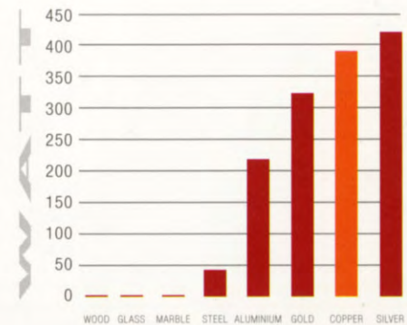
METAL CONDUCTIVITY CHART
